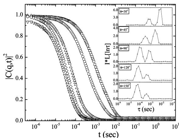
Figure 3. Intensity autocorrelation functions of a 0.1 wt % solution of PHEGMA 50 - b -PDEAEMA 50 at degree of ionization \alpha = 0.1 and scattering angles 30° ( \square ), 45° ( \circ ), 90° ( \triangle ), 120° ( \diamond ), and 150° ( \nabla ). The distributions of relaxation times multiplied by the total scattering intensity (normalized to that of toluene) are shown in the insets for the respective scattering angles.
