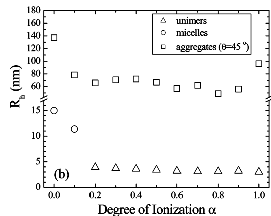
Figure 5. Scattering intensities normalized to that of toluene (a) and hydrodynamic radii (b) of a 0.1 wt % PHEGMA 50 - b -PDEAEMA 50 diblock copolymer solution as a function of the degree of ionization \alpha of the PDEAEMA block.
