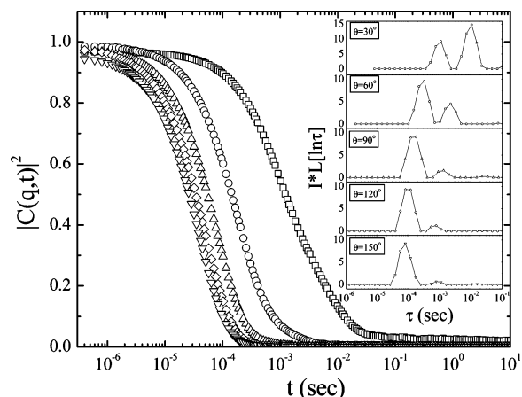
Figure 4. Intensity autocorrelation functions of a 0.1 wt % solution of PHEGMA 50 - b -PDEAEMA 50 at degree of ionization \alpha = 0 and scattering angles 30° ( \square ), 60° ( \circ ), 90° ( \triangle ), 120° ( \diamond ), and 150° ( \nabla ). The distributions of relaxation times multiplied by the total scattering intensity (normalized to that of toluene) are shown in the insets for the respective scattering angles.
